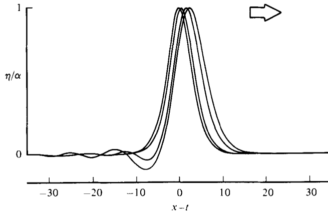
FIGURE 9. Computed, normalized profiles shown as a function of s at times t = 26, 51, 101, 151 (from left to right) for a wave of amplitude \alpha_0 = 0.1 in a diverging channel (cf. figure 8).
