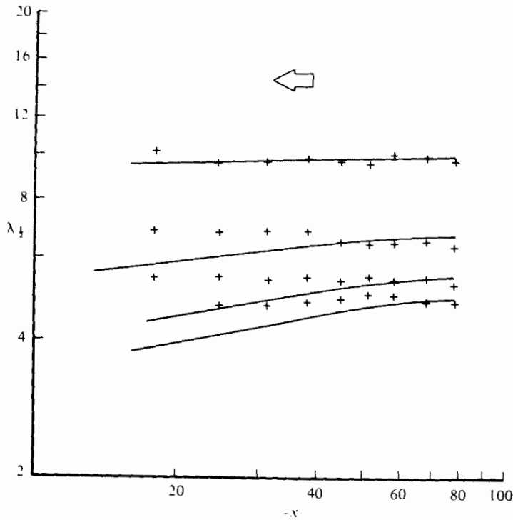
FIGURE 5. Measured (+) and computed (—) halfwidths corresponding to the amplitudes shown in figure 4.
