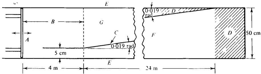
FIGURE 1. Plan view of the wave channel (not to scale). A , bulkhead wave-maker. B , entrance section. C , diagonal wall. D , wave-damping material. E , glass sidewalls. F , diverging channel. G , converging channel.
