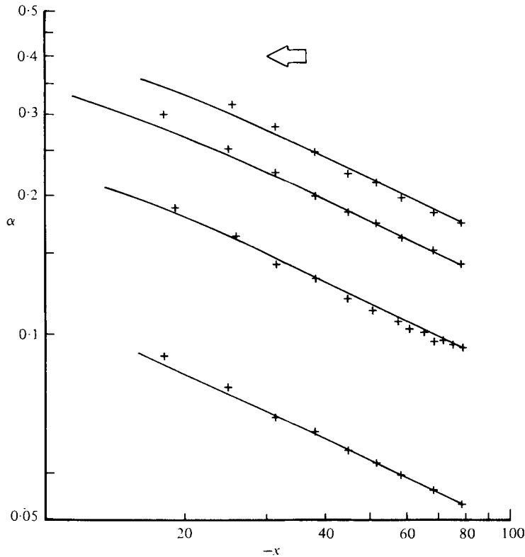
FIGURE 4. Measured (+) and computed (—) amplitudes of solitary waves in a converging channel of convergence angle 0.019 rad and 30 cm depth. The initial amplitudes are \alpha_0 = 0.043, 0.093, 0.140, 0.174 .
