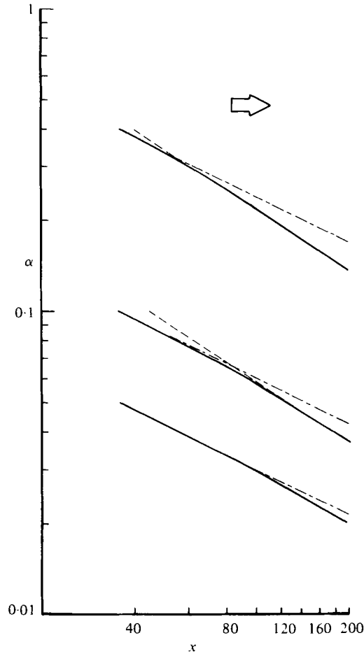
FIGURE 8. Amplitude vs. position ( \alpha vs. x ) of computed profiles of solitary waves of amplitude \alpha_0 = 0.05, 0.1, 0.4 in a diverging channel: t_0 = 36 . Also shown are the lines of slope -\frac{1}{2} (---), -\frac{2}{3} (-·-·).
