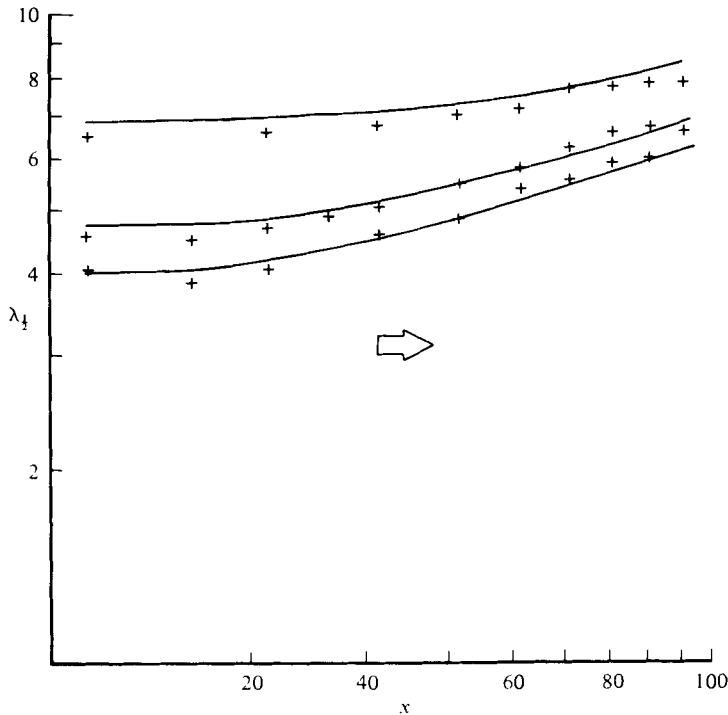
FIGURE 3. Measured (+) and computed (—) halfwidth, \lambda_{\frac{1}{2}} , corresponding to the amplitudes shown in figure 1.
