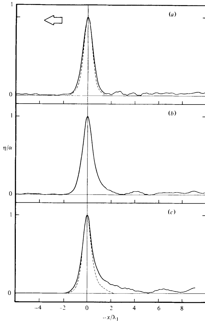
FIGURE 7. Measured normalized profiles of a solitary wave of initial amplitude \alpha_0 = 0.2 in a converging channel of 40 cm depth at stations (a) x_0 = -58.5 , (b) x = -43.5 , (c) x = -23.5 . The broken lines in (a) and (c) show the corresponding initial data and subsequent numerical solution of equation (3.1).
