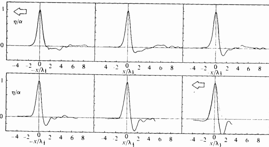
FIGURE 6. Measured temporal profiles (—) and Boussinesq profiles (---) for \alpha_0 = 0.4 in a diverging channel of 30 cm depth. The profiles were measured at x = 4.2, 17.6, 30.9, 37.6, 50.9, 64.3 .
