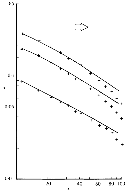
FIGURE 2. Measured (+) and computed (—) amplitudes, \alpha , of solitary waves in a diverging channel of expansion angle 0.019 rad and 20 cm depth. The initial amplitudes are \alpha_0 = 0.088, 0.185, 0.259 . Note that \alpha and x are normalized with respect to the quiescent depth.
