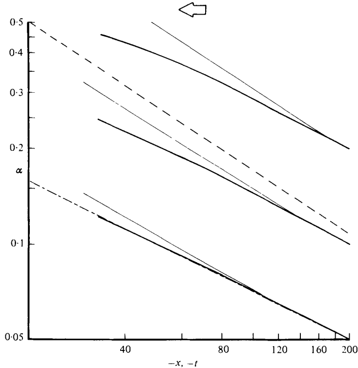
FIGURE 10. Amplitude \alpha vs. position x (—) and time t (—) of computed profiles of solitary waves of amplitude \alpha_0 = 0.05, 0.1, 0.2 in a converging channel: x_0 = t_0 = 200 . Also shown are lines of slope -\frac{1}{2} (---), and -\frac{2}{3} (---). Note the increasing divergence of the temporal and spatial curves with increasing wave amplitude.
