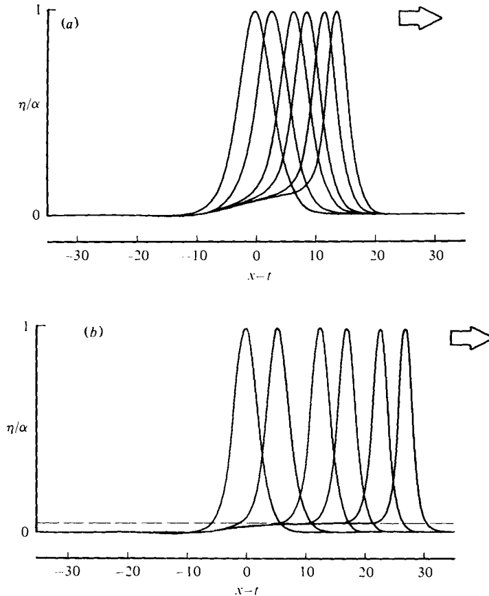
FIGURE 11. Computed, normalized profiles shown as a function of s at times t = -200, -150, -100, -75, -50, -35 (from left to right) for waves of amplitude (a) \alpha_0 = 0.1 , (b) \alpha_0 = 0.2 . The broken line in (b) is the amplitude of the shelf predicted by equation (1.7) (cf. figure 10). [It should be noted that the amplitude of the shelf predicted by (1.7) varies as b^{-1} and that the amplitude used to normalize these profiles (cf. figure 10) differs negligibly from the -\frac{1}{2} -power law over most of the range shown here. The maximum difference (of approximately 6% at t = -35 ) is not discernible on the scale of this figure.]
